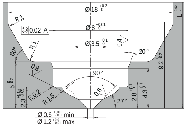
Tip style 1B15-PK - Cutout dimensions
