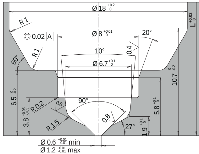
Tip style 1B50-PK - Cutout dimensions
