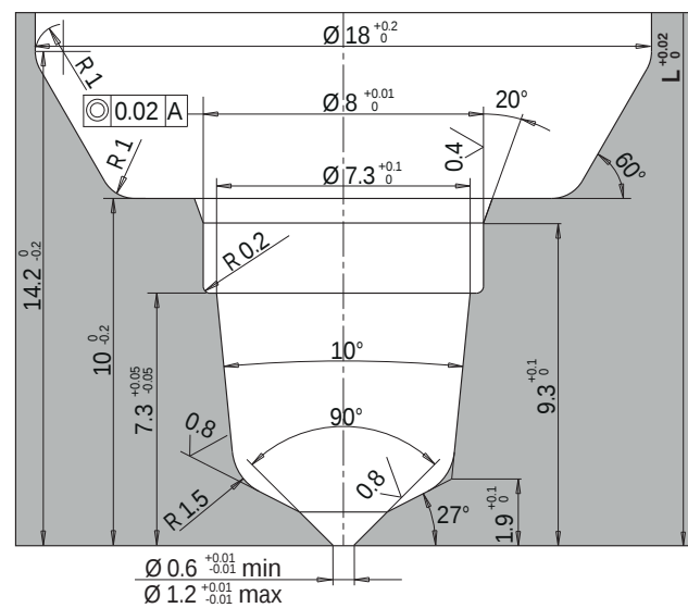
Tip style 1B50-PK - Cutout dimensions
